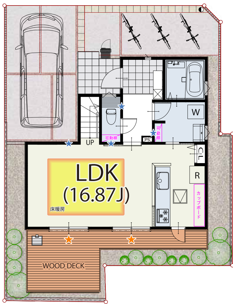
1 FLOOR / 45.13㎡
